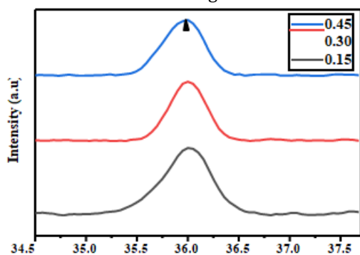
Fig. 3 XRD patterns indicate a slight shift towards lower angle
