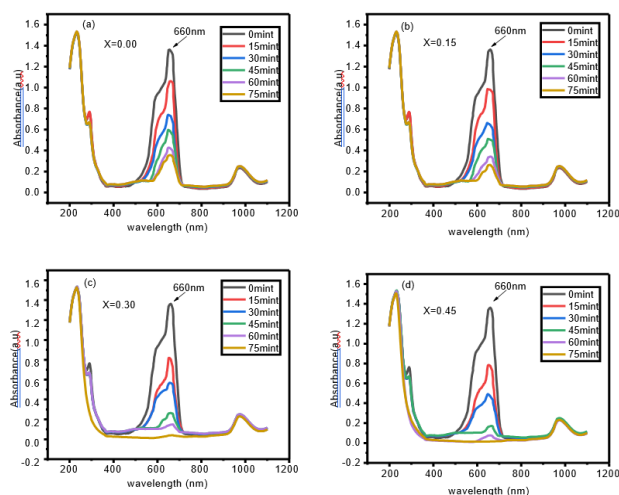
Fig. 10 MB degradation spectrums of a) pure NF b) CNF x=0.15 , c) CNF x=0.30 , and d) CNF x=0.45
