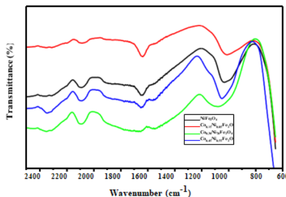
Fig. 5 FTIR spectrums of NF and Co-doped NiFe 2 O 4
