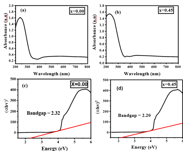
Fig. 6 Uv-Vis spectra of a) NF and b) CNF ( x=0.45 ), Tauc's plot acquired for c) NF and d) CNF ( x=0.45 )
