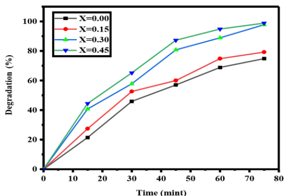
Fig. 9 Degradation percentage of MB
