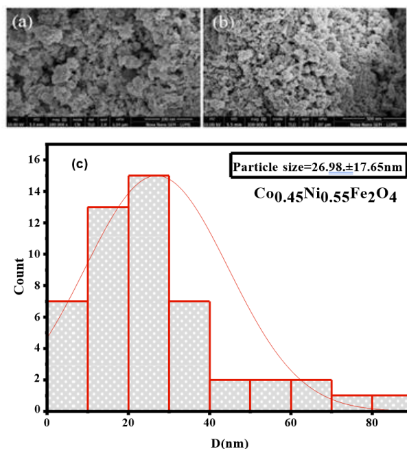
Fig. 8 (a, b) SEM images of CNF ( x=0.45 ), (c) Statistical histogram of size distribution of CNF ( x=0.45 )
