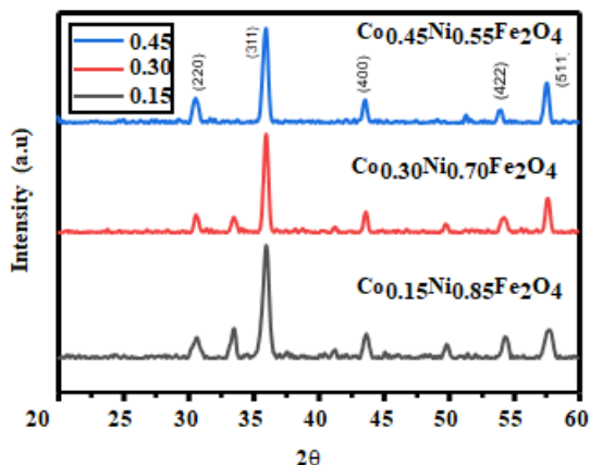
Fig. 3 XRD patterns indicate a slight shift towards lower angle
