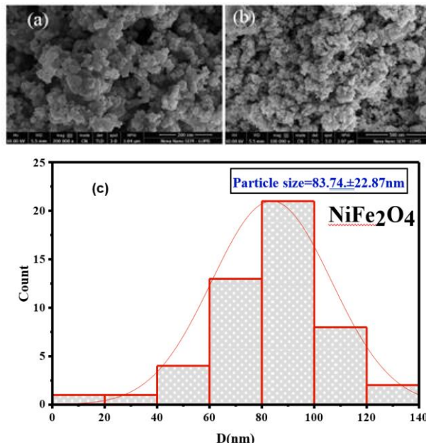
Fig. 7 (a, b) SEM images of \text{NiFe}_2\text{O}_4 , (c) Statistical histogram of size distribution of \text{NiFe}_2\text{O}_4
