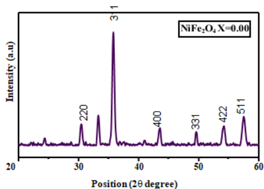
Fig. 1 XRD pattern of NiFe 2 O 4
