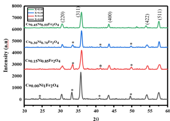
Fig. 2 XRD patterns of Co doped NiFe 2 O 4
