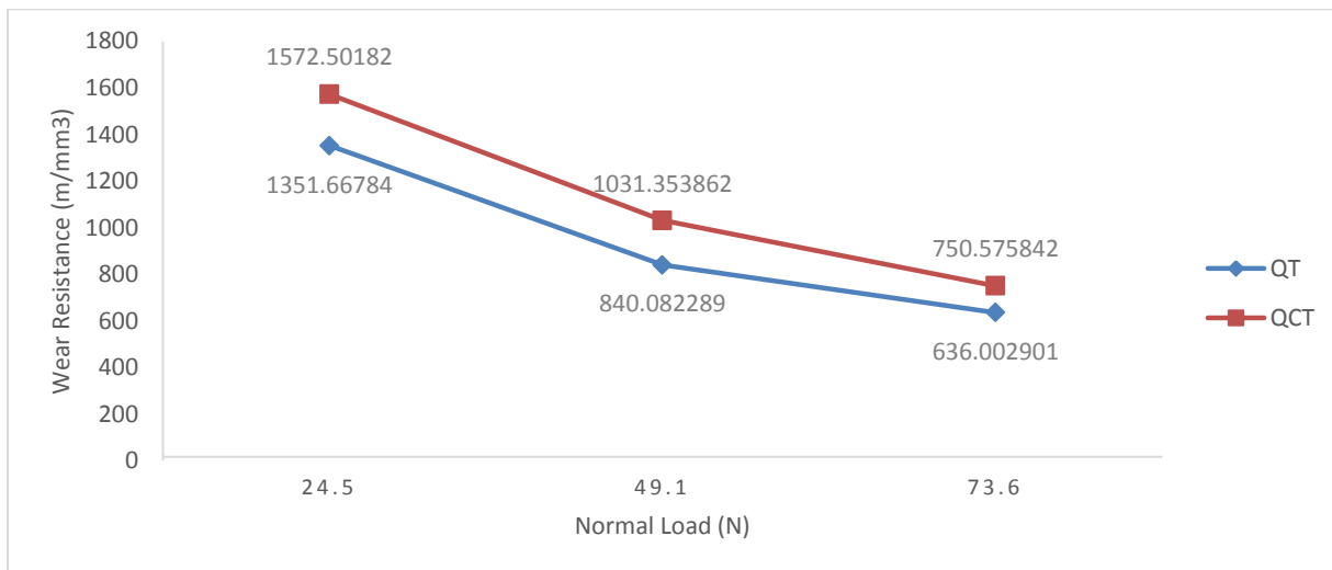
Fig.2: Graph Showing variation of wear resistance along with variation of load at sliding velocity 1.0 m/s
