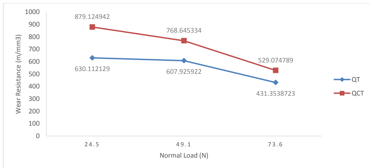
Fig.4 Graph showing variation of wear resistance along with variation of load at sliding velocity 2.0 m/s
