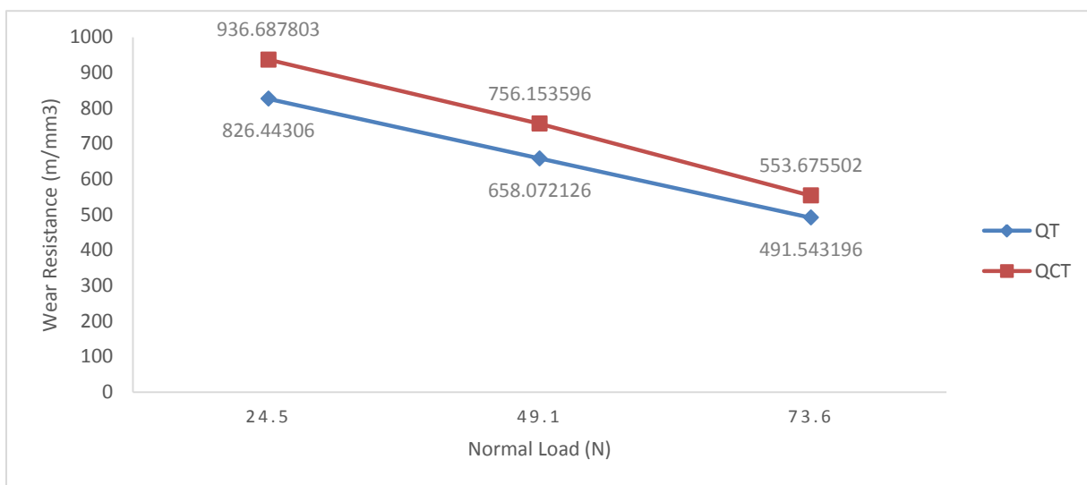
Fig. 3: Graph showing variation of wear resistance along with variation of load at sliding velocity 1.5 m/s
