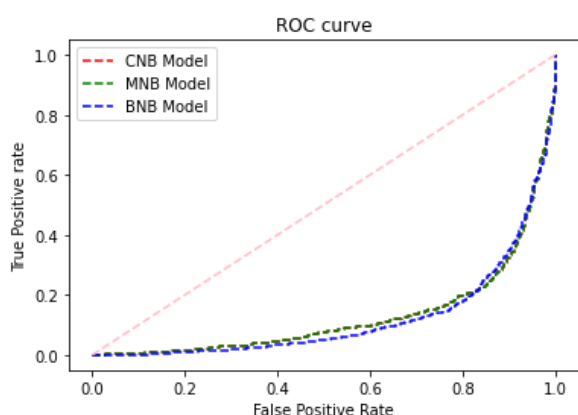
Figure 4 The Graph the Receiver Operating Characteristic (ROC)
