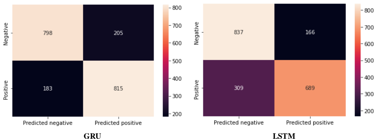
Figure 10 Confusion Matrices of the GRU and LSTM Classifier
