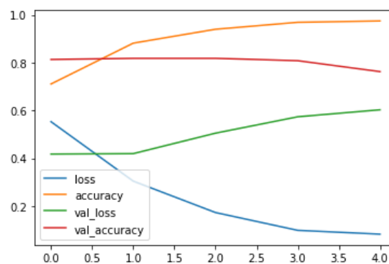
LSTM
