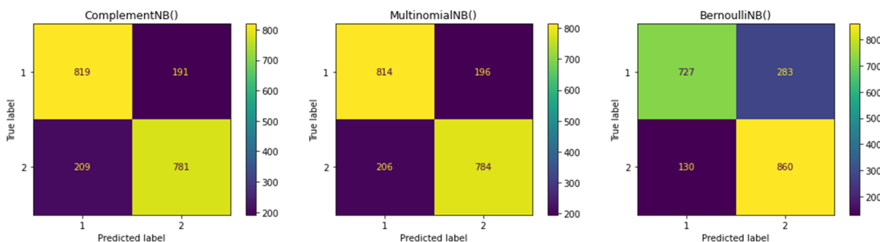
Figure 3 Confusion Matrices of the different NB Classifier
