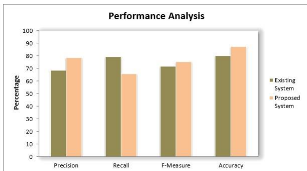
Fig. 2. Analysis Graph
