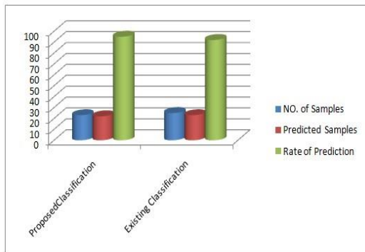
Fig. 2. Classification graph
