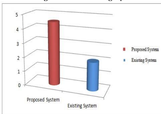
Fig. 3. Algorithms Comparison
