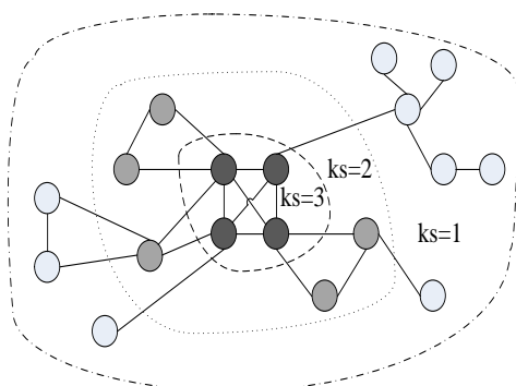
Figure 2 A simple network with three shells
