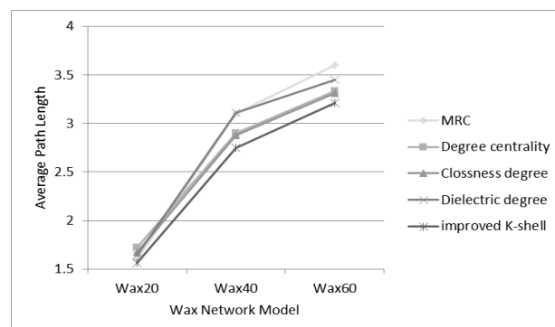
Figure 4 The path length of Wax network single link failure
