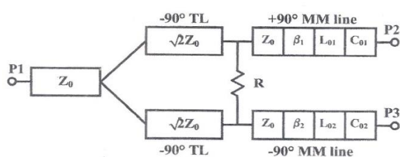
Fig. 5 (b) The architecture of the NRI-TL balun
