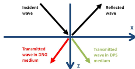
Fig. 4: Geometry of the scattering of a wave obliquely incident upon a DPS-DNG interface
