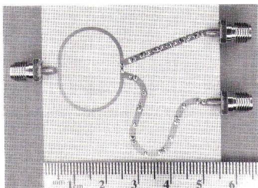
Fig. 5 (a) A photograph of the fabricated NRI-TL balun in microstrip
