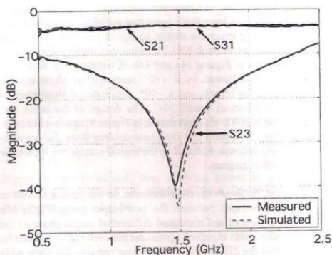
Fig. 6 (a) The measured and simulated isolation (S 23 ) and through (S 21 and S 31 ) magnitude responses of the NRI-TL balun
