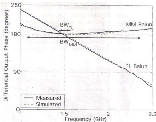
Fig. 6 (b) The measured and simulated differential phase comparison between the NRI-TL balun and the transmission-line balun
