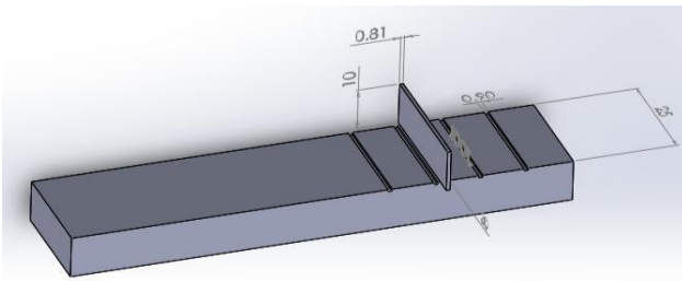
Figure 1: Schematic of workpiece and electrode sheet
