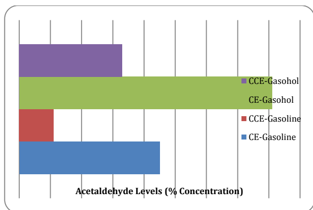
Fig.3 Bar charts showing the variation of Acetaldehyde levels with different versions of the engine with test fuels
