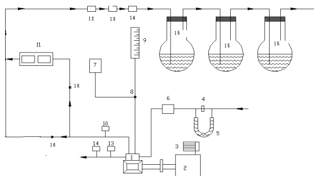
1.Engine, 2.Eddy current dynamometer, 3. Loading arrangement, 4. Orifice meter, 5. U-tube water monometer, 6. Air box, 7. Fuel tank, 8. Three-way valve, 9. Burette, 10. EGT Indicator, 11. Catalytic converter, 12. Filter, 13. Rotometer, 14. Heater, 15. Round bottom flask containing DNPH solution 16. Directional valve.
