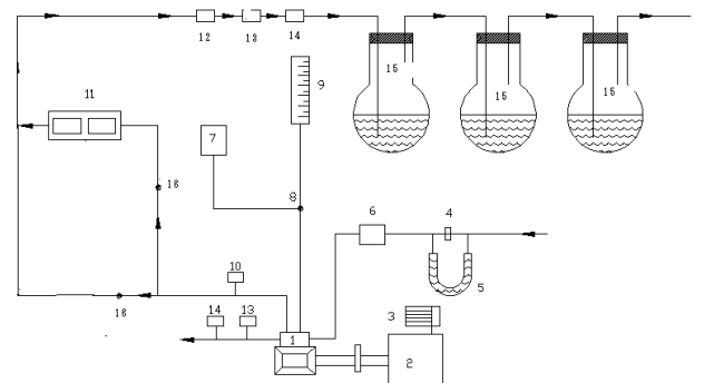
1.Engine, 2.Eddy current dynamometer, 3. Loading arrangement, 4. Orifice meter, 5. U-tube water monometer, 6. Air box, 7. Fuel tank, 8. Three-way valve, 9. Burette,10. EGT Indicator, 11. Catalytic converter, 12.Filter, 13. Rotometer, 14.Heater, 15. Round bottom flask containing DNPH solution 16. Directional valve.
