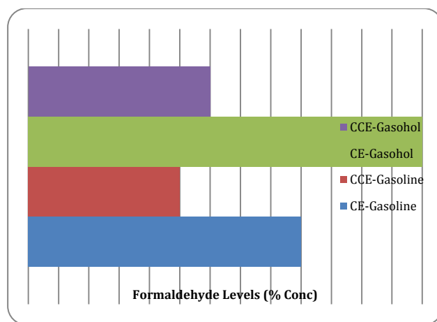
Fig.2 Bar charts showing the variation of formaldehyde levels with different versions of the engine with test fuels
