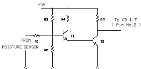
Fig 2.4 Signal Conditioning Circuit for Moisture Measurement
