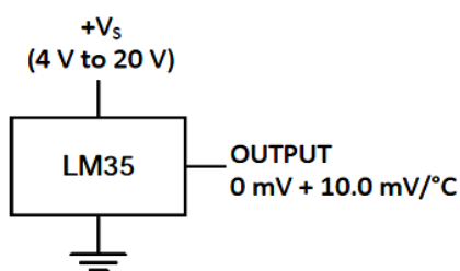
Figure 2.4: Basic Centigrade Temperature Sensor (+2°C to +150°C)
