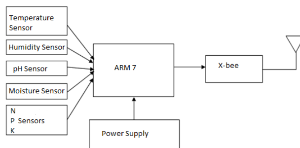
Figure 2.2 Wireless sensor node
