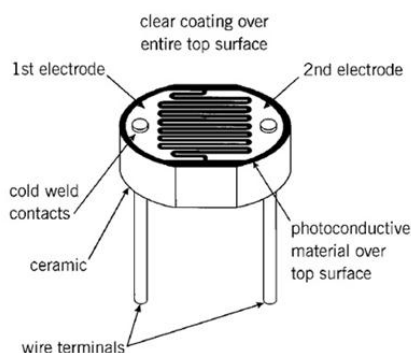
Fig 2.8 LDR Sensor
