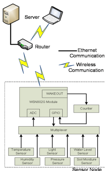
Figure 2.1: Functional Block diagram of System being developed
