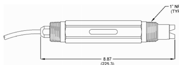
Fig 2.7 pH sensor
