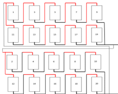
Fig. 4 Solar cell connection
