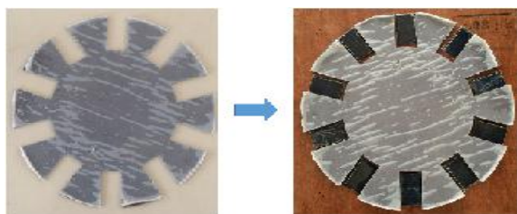
Fig.3 Disc Arrangement
