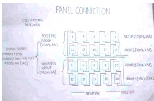
Fig. 6 230V Calculations
