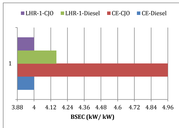
Fig.4 Bar charts showing the variation of brake specific energy consumption (BSEC) with conventional engine and LHR-1 engine with neat diesel and crude jatropha oil operation at 27° bTDC and injection pressure of 190 bar
