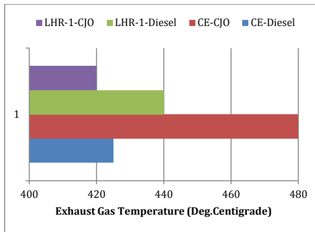
Fig.5. Bar charts showing the variation of exhaust gas temperature with conventional engine and LHR-1 engine with neat diesel and crude jatropha oil operation at 27° bTDC and injection pressure of 190 bar
