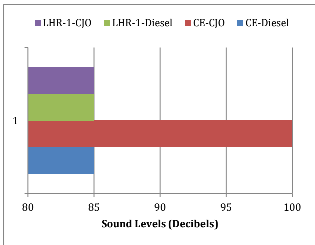
Fig.7 Bar charts showing the variation of sound levels with conventional engine and LHR-1 engine with neat diesel and crude jatropha oil operation at 27° bTDC and injection pressure of 190 bar
