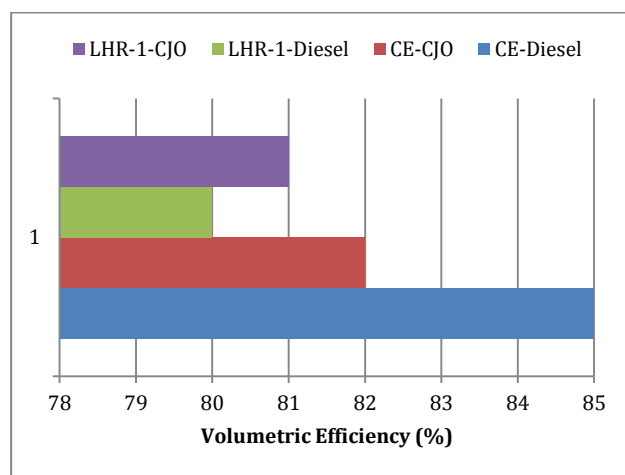
Fig. 8 Bar charts showing the variation of volumetric efficiency with conventional engine and LHR-1 engine with neat diesel and crude jatropha oil operation at 27° bTDC and injection pressure of 190 bar
