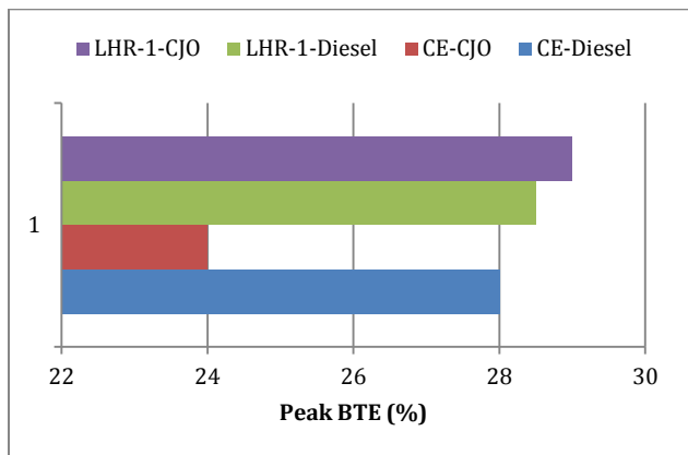
Fig.3 Bar charts showing the variation of peak BTE with conventional engine and LHR-1 engine with neat diesel and crude jatropha oil operation at 27 °bTDC and injection pressure of 190 bar
