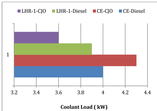
Fig.6 Bar charts showing the variation of coolant load with conventional engine and LHR-1 engine with neat diesel and crude jatropha oil operation at 27° bTDC and injection pressure of 190 bar
