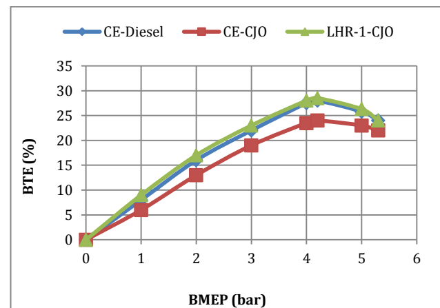
Fig.2 Variation of brake thermal efficiency (BTE) with brake mean effective pressure (BMEP) in conventional engine (CE) and LHR-1 engine with crude jatropha oil (CJO) operation at 27^\circ bTDC and at an injector opening pressure of 190bar
