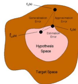
Fig.2 Statistical Learning Theory
