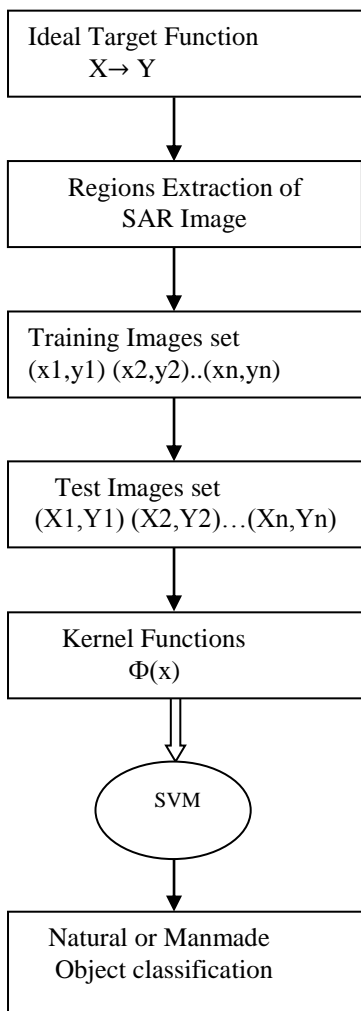
Fig 7: Algorithm flow of Object Classification
