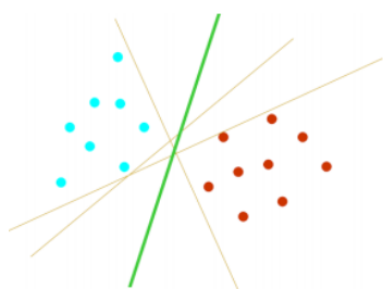
Fig.3 Optimal Separating Hyperplane
