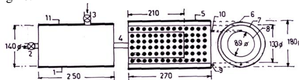
1.Air chamber, 2.Inlet for air chamber from the engine, 3.Inlet for air chamber from compressor, 4.Outlet for air chamber, 5.Catalyst chamber, 6. Outer cylinder, 7. Intermediate cylinder, 8.Inner cylinder, 9. Outlet for exhaust gases, 10.Provision to deposit the catalyst and 11.Insulation
