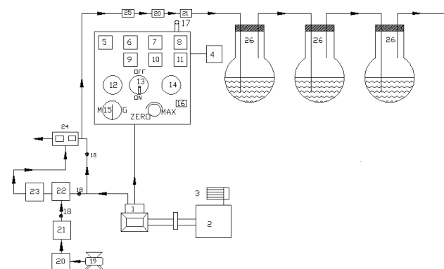
1. Engine, 2.Electrical swinging field dynamometer, 3. Loading arrangement, 4.Fuel tank, 5.Torque indicator/controller sensor, 6. Fuel rate indicator sensor, 7. Hot wire gas flow indicator, 8. Multi channel temperature indicator, 9. Speed indicator, 10. Air flow indicator, 11. Exhaust gas temperature indicator, 12. Mains ON, 13. Engine ON/OFF switch, 14. Mains OFF, 15. Motor/Generator option switch, 16. Heater controller, 17. Speed indicator, 18. Directional valve, 19. Air compressor, 20. Rotometer, 21. Heater, 22. Air chamber, 23. Catalytic chamber, 24. CO/HC analyzer, 25. Filter, 26. Round bottom flasks containing DNPH solution,
