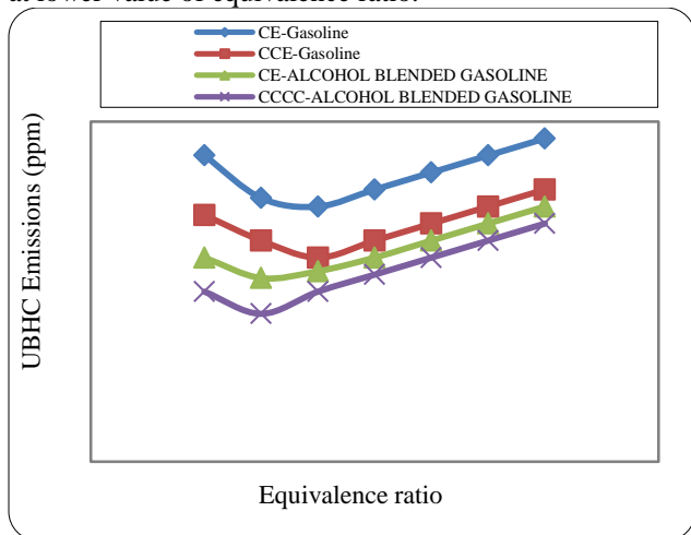
CE- conventional engine: CCCC-Copper coated combustion chamber, UBHC-Un-burnt hydro carbons
