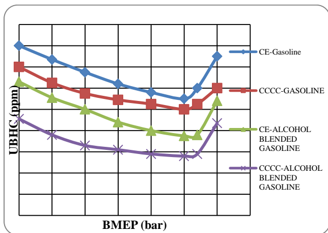
CE-conventionalengine: CCCC-Copper coated combustion chamber, UBHC- Un-burnt hydro carbons: BMEP-Brake mean effective pressure
