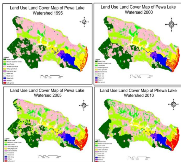
Figure 2 LULC classifications for years 1995, 2000, 2005 and 2010
