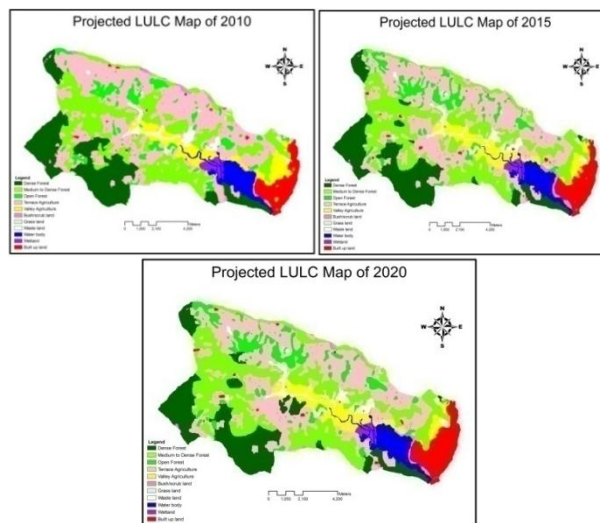
Figure 4 Predicted LULC maps for 2010, 2015 and 2020
