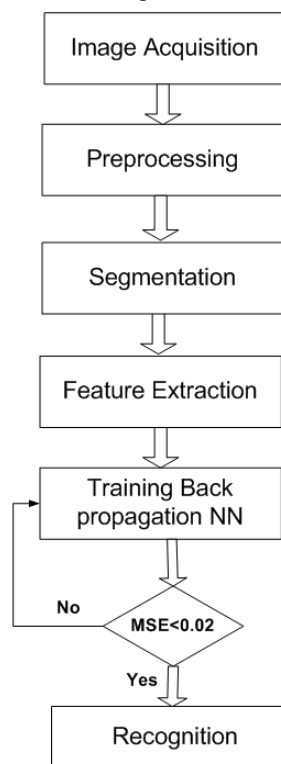
Fig.1 East Syriac Character Recognition System
