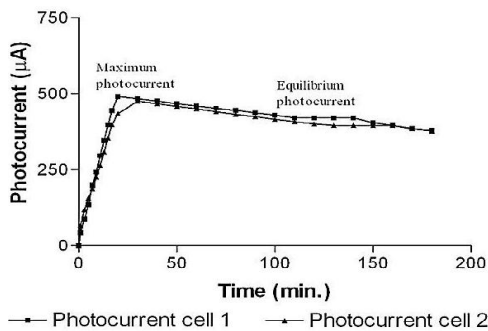
Figure 4 Variation of Photocurrent with Time in Cell I & II Methylene blue-EDTA-TX 100 & Azur B-EDTA-CTAB system respectively.
