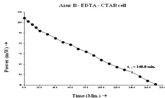
Figure-5 Performance of the photogalvanic cell
