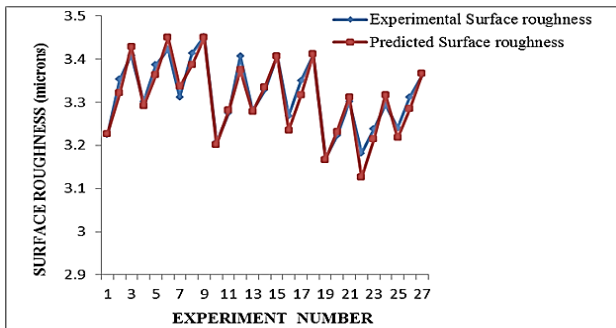
Fig. 3 Comparison plot of surface roughness obtained from the Taguchi DOE and RSM.
