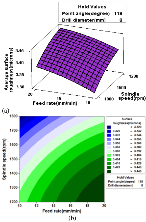
Fig. 5 Interaction effects of feed rate and spindle speed on surface roughness
