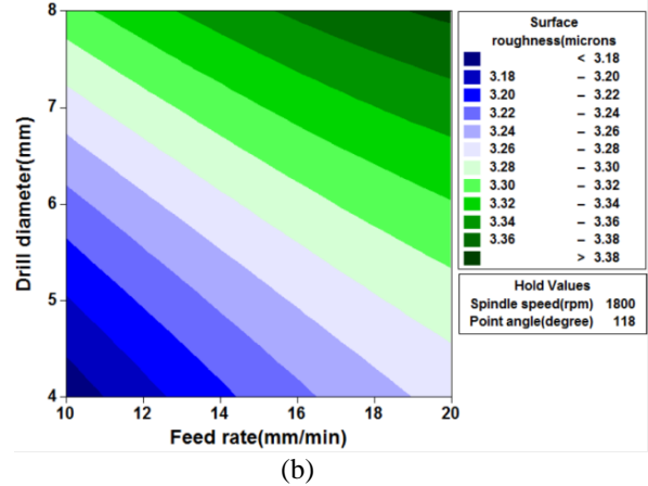
Fig.6 Interaction effects of feed rate and drill diameter on surface roughness
