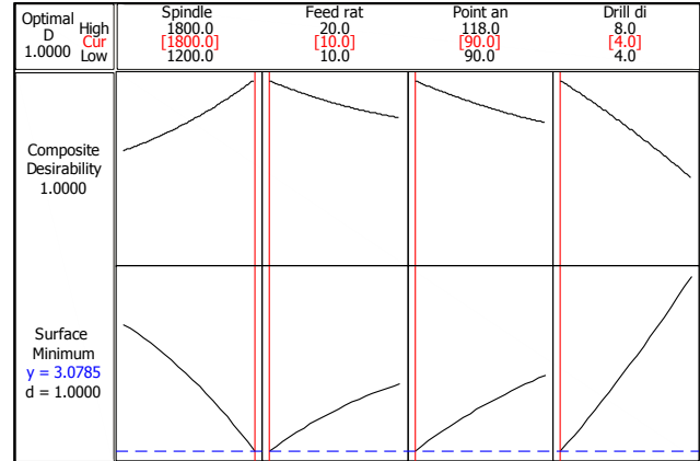
Fig. 9 Optimized response surface plot of surface
