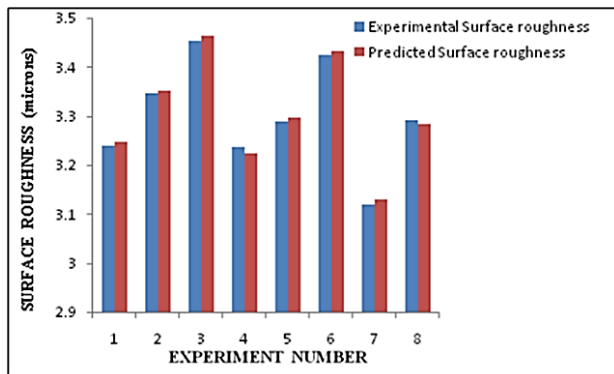
Fig.10 Comparison of the experimental and the predicted values of surface roughness
