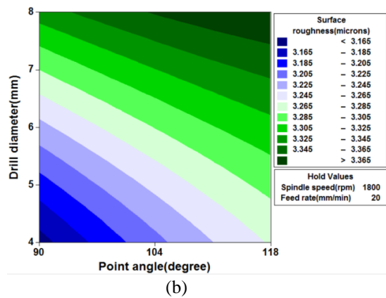
Fig.7 Interaction effects of point angle and drill diameter on surface roughness
