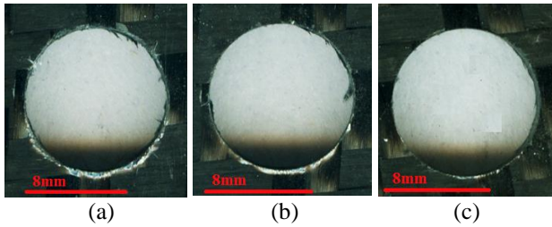
Fig.8 Delamination obtained for (a) 1200rpm, 20mm/min, 118degree (b) 1500rpm, 20mm/min, 90degree (c) 1800rpm, 20mm/min, 104degree
