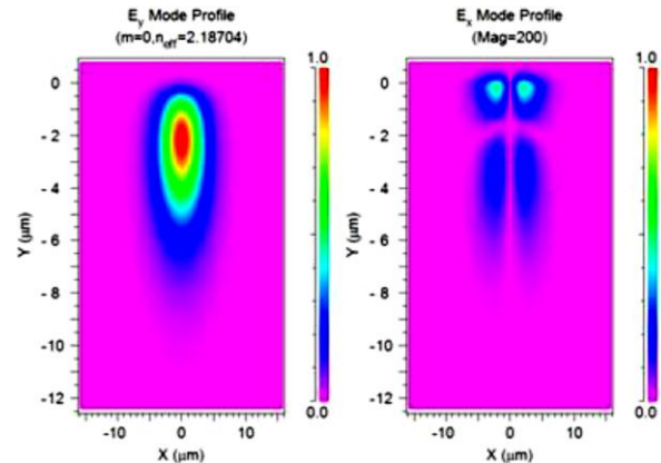
Fig3: Simulation of the Mode profile and effective refractive index across the width of the optical splitter at the wavelength 1550nm, Width 6µm.
