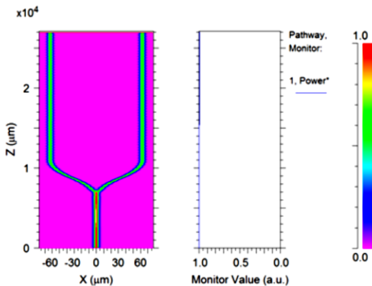
Fig 2: Simulation of optical signal in power splitter
