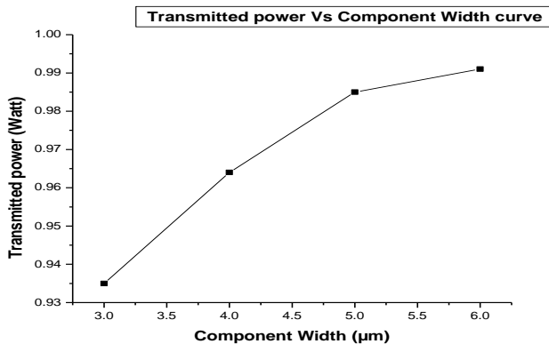
Fig 4 Transmitted power v/s Component width
