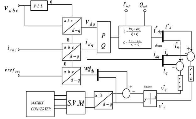
Fig 5:Control system of series part of proposed unified power quality conditioner
