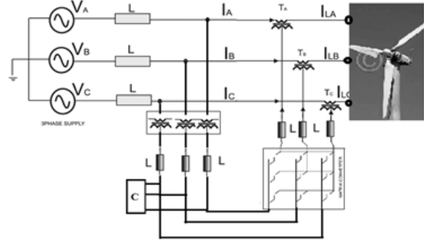
Fig 3: Proposed unified power quality conditioner
