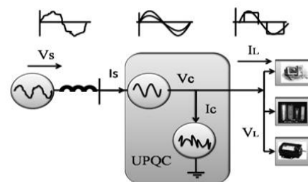
Fig 1: basic structure of unified power quality conditioner
