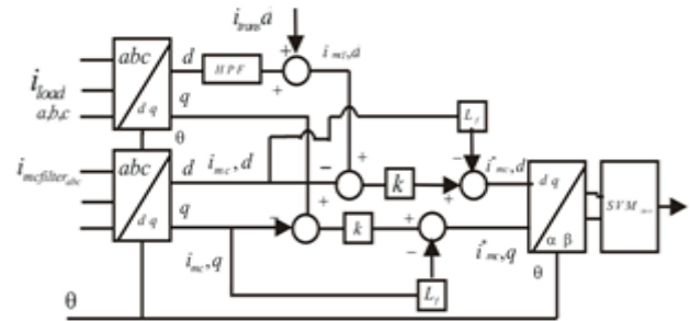
Fig 6:Control system of shunt part of proposed unified power quality conditioner
