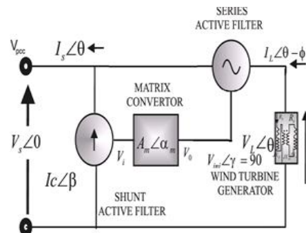
Fig 4: fundamental diagram of proposed unified power quality conditioner connected to an induction wind turbine Generator
