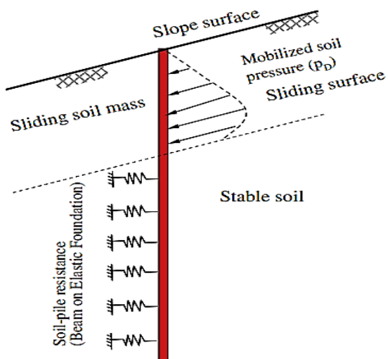
Figure 6: Proposed model for soil-pile analysis in pile stabilized slopes (Ashour and Ardalán, 2012)
