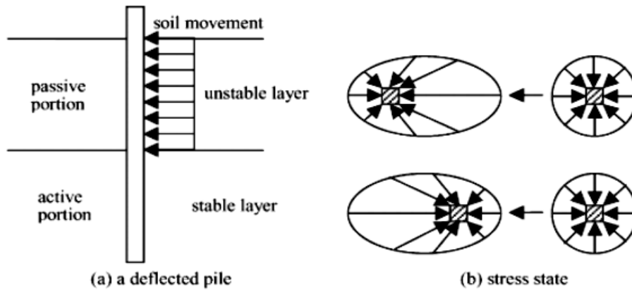
Fig. 3 A pile undergoing lateral soil movement – (a) A deflected pile; (b) Stress state (after Jeong et al., 2003).
