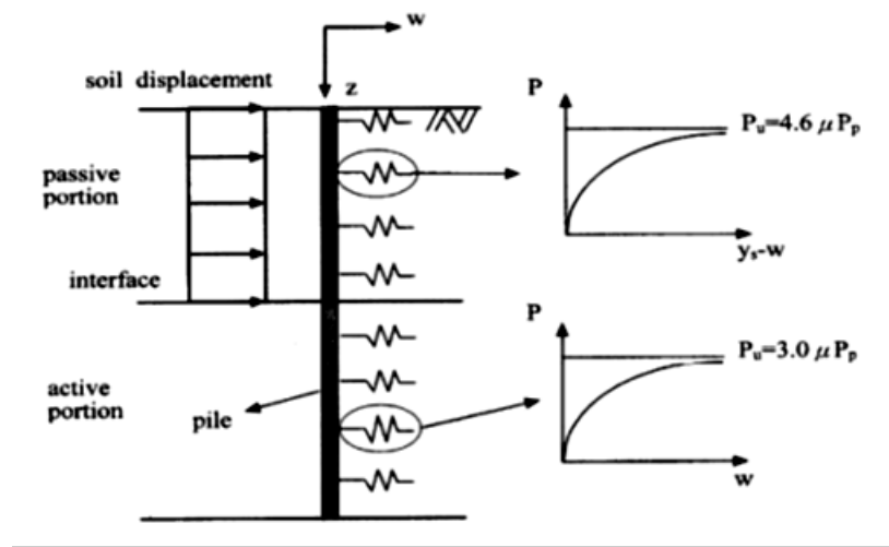
Fig. 4 A pile subjected to lateral soil displacement (after Jeong et al., 2003).
