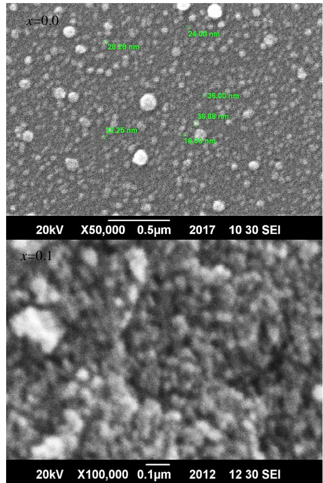
Figure.4 SEM images for \text{CoGd}_x\text{Fe}_{2-x}\text{O}_4 ( x=0.0 ) and ( x=0.1 ) nanoparticles synthesized by sol-gel auto combustion method
