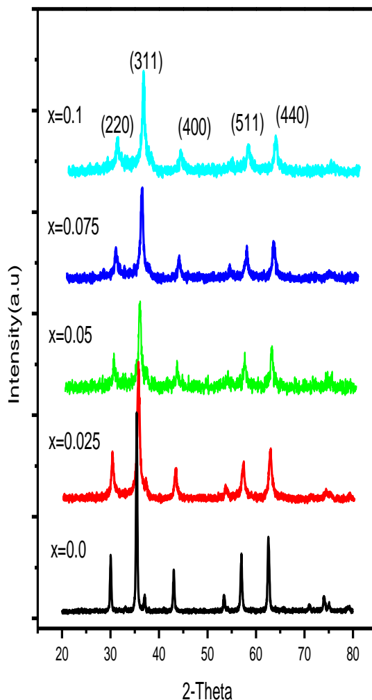
Figure.1 Indexed XRD patterns of CoGd_xFe_{2-x}O_4 ( x=0.0 to x=0.1 ) nanoparticles synthesized by sol-gel auto combustion method
