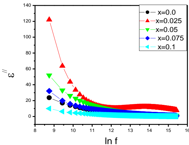
Figure.8 Variations of Permittivity \epsilon'' (imaginary part) with \ln f for \text{CoGd}_x\text{Fe}_{2-x}\text{O}_4 ( x=0.0 to x=0.1 ) nanoparticles synthesized by sol-gel auto combustion method
