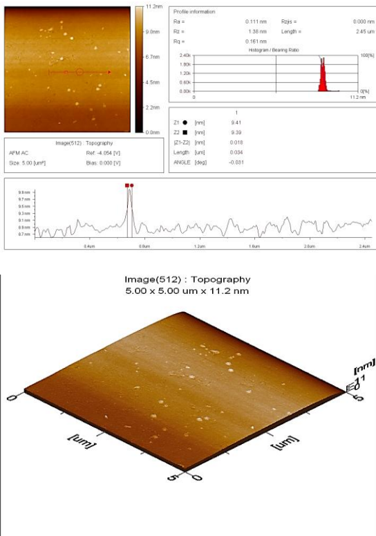
Fig.5 AFM micrograph for \text{CoGd}_x\text{Fe}_{2-x}\text{O}_4 ( x=0.025 ) nanoparticles synthesized by sol-gel auto combustion method
