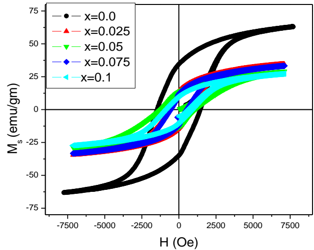
Figure.12 (a) M-H loops for CoGd_xFe_{2-x}O_4 ( x=0.0 to x=0.1 )
