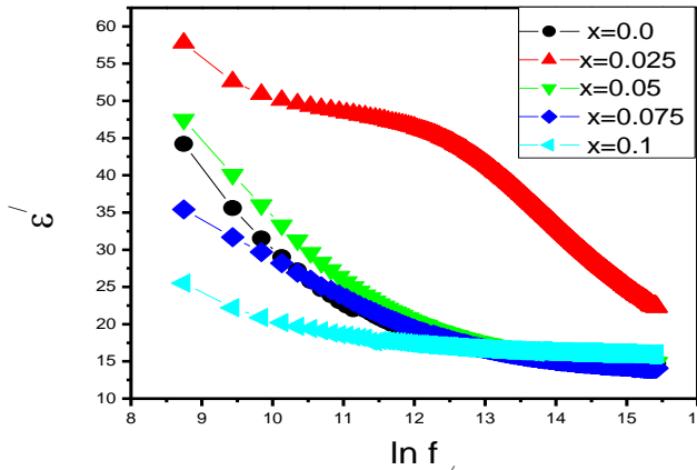
Figure.7 Variations of Permittivity \epsilon' (real part) with \ln f for \text{CoGd}_x\text{Fe}_{2-x}\text{O}_4 ( x=0.0 to x=0.1 ) nanoparticles synthesized by sol-gel auto combustion method
