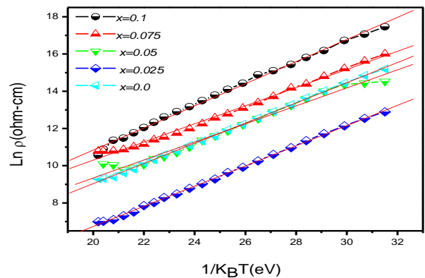
Figure.6 (b) Variation of DC electrical resistivity ( \ln \rho ) with inverse of temperature 1/K_B T (eV) for \text{CoGd}_x\text{Fe}_{2-x}\text{O}_4 ( x=0.0 to x=0.1 ) nanoparticles synthesized by sol-gel auto combustion method
