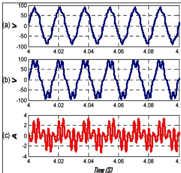
Fig. 4 Grid connected voltage controlled DG without flicker compensation (a) PCC voltage (b) DG phase voltage (c) DG current
