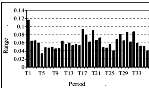
Fig. 7 Flicker range when DG is connected at the beginning of monitoring period
